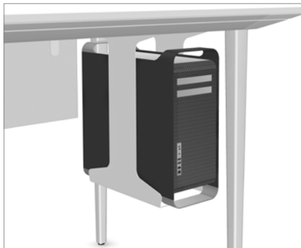
CPU holder. 25-30x49 cm and 1,5 mm thick sheet steel
